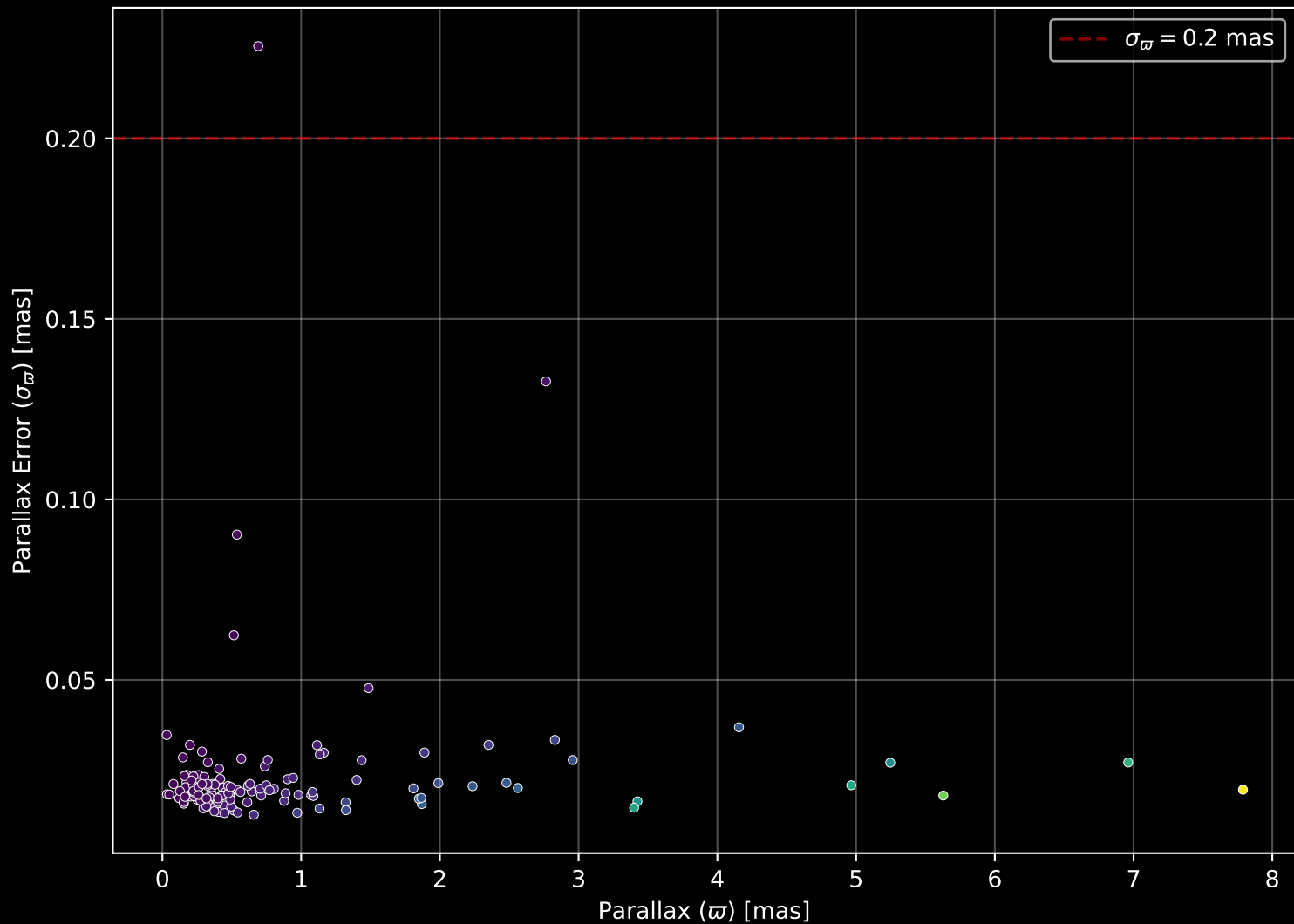
APOGEE DR17 Field: [015+30] Parallax Quality (n= 135)
