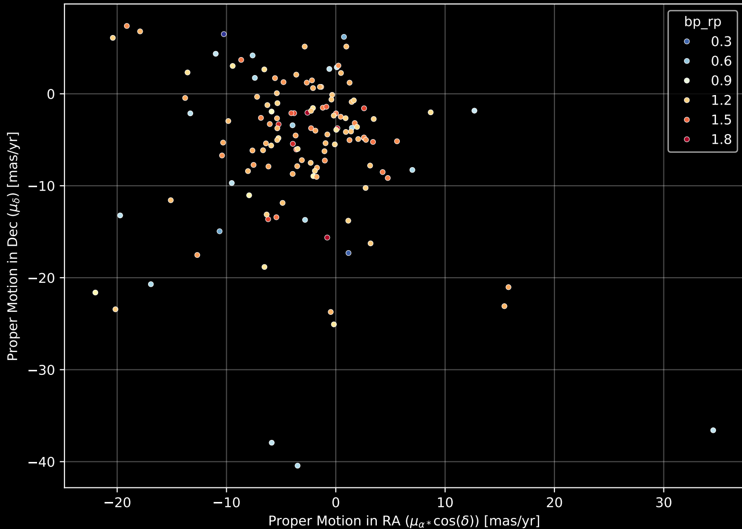
APOGEE DR17 Field: [015+30] Proper Motion Diagram (n= 135)
