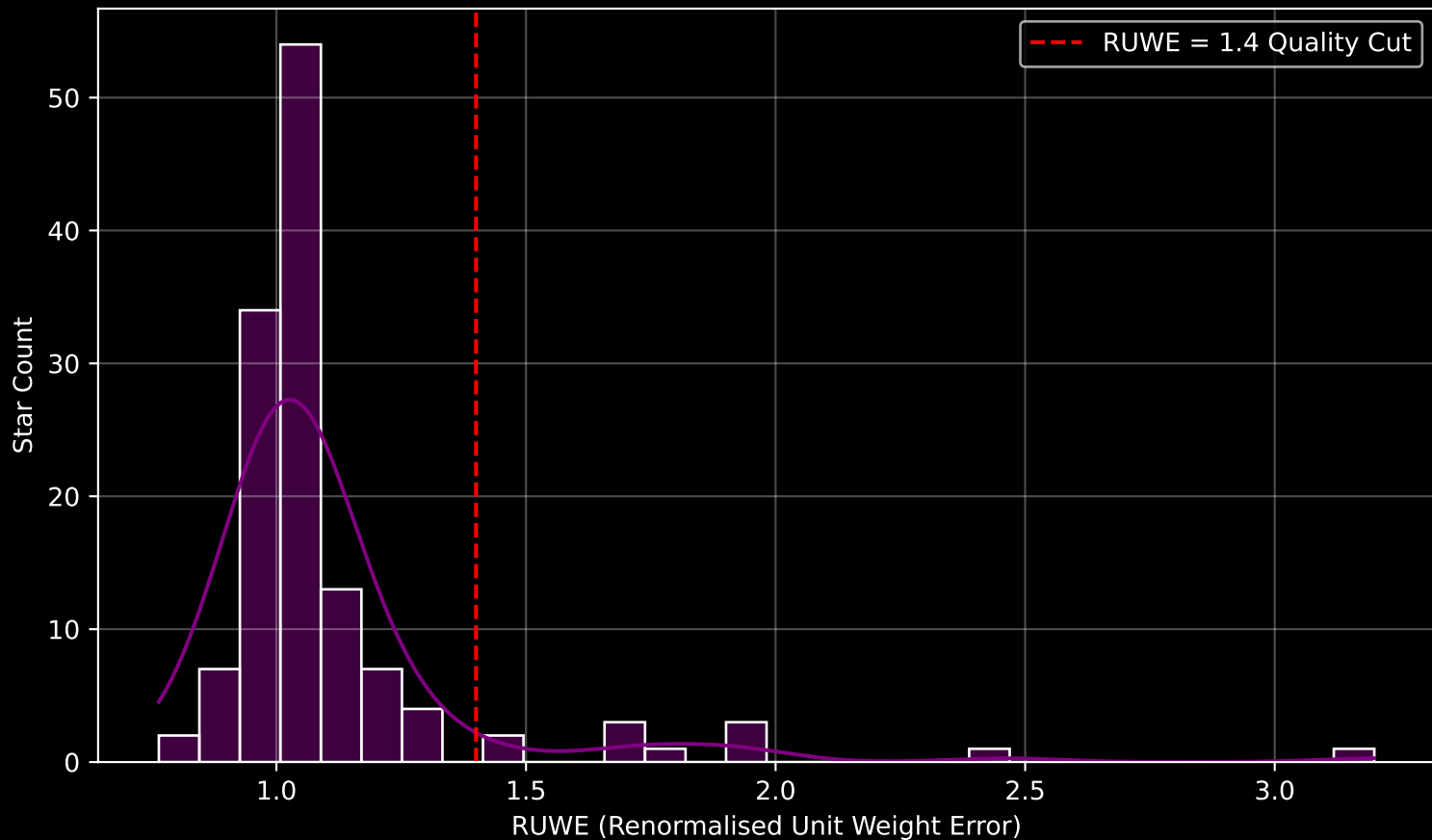
GAPOGEE DR17 Field [015+30] RUWE Distribution (n= 132)
