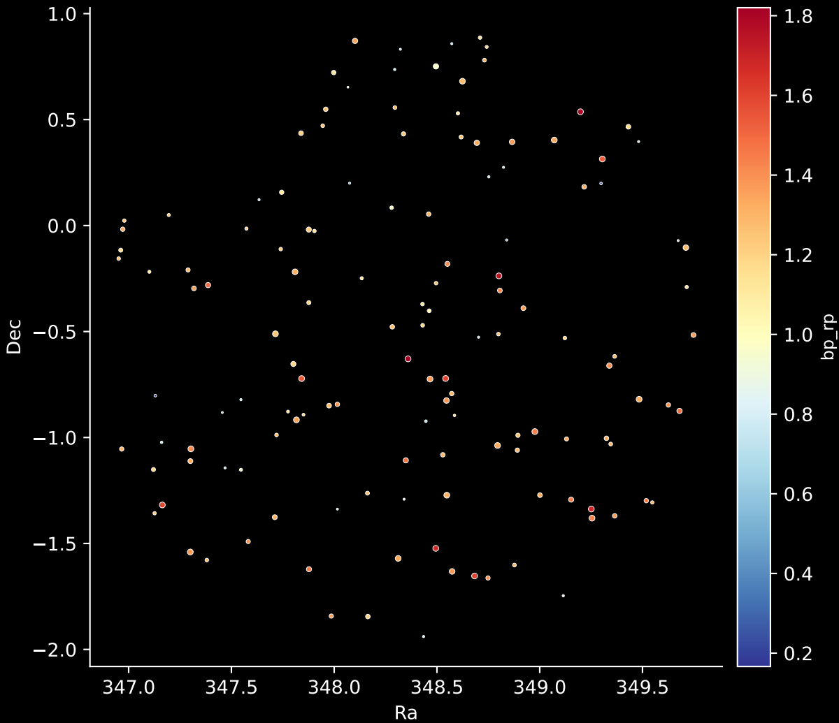
APOGEE DR17 Field: [015+30] Stars: 135
