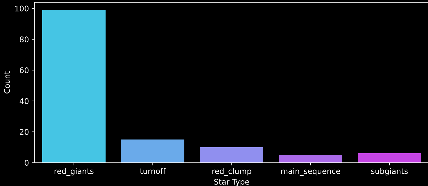
APOGEE DR17 Field: [015+30] Count plot of Star Type
