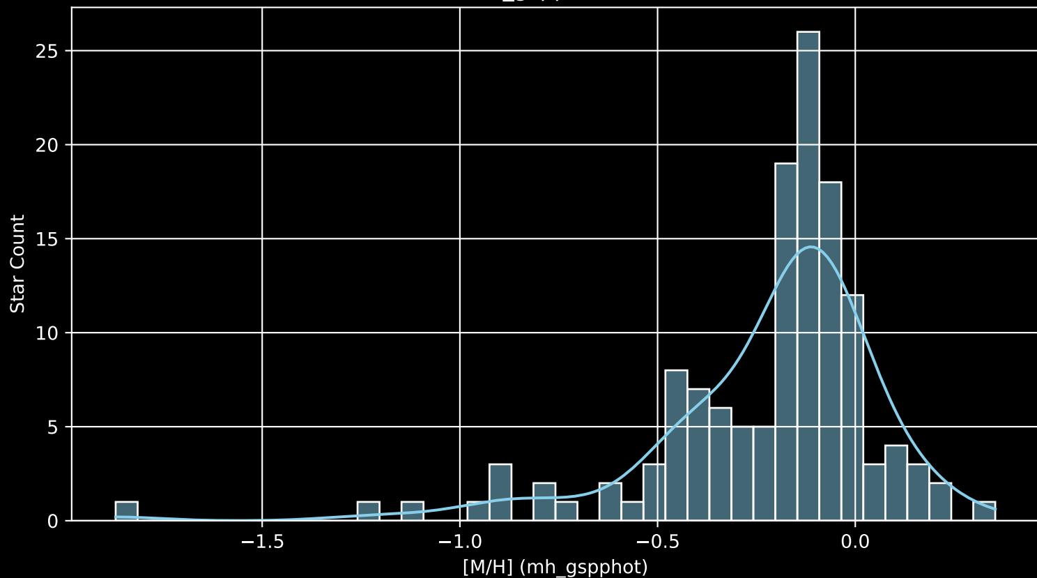
APOGEE DR17 Field: [015+30 [M/H] (mh_gspphot) (n= 135)
