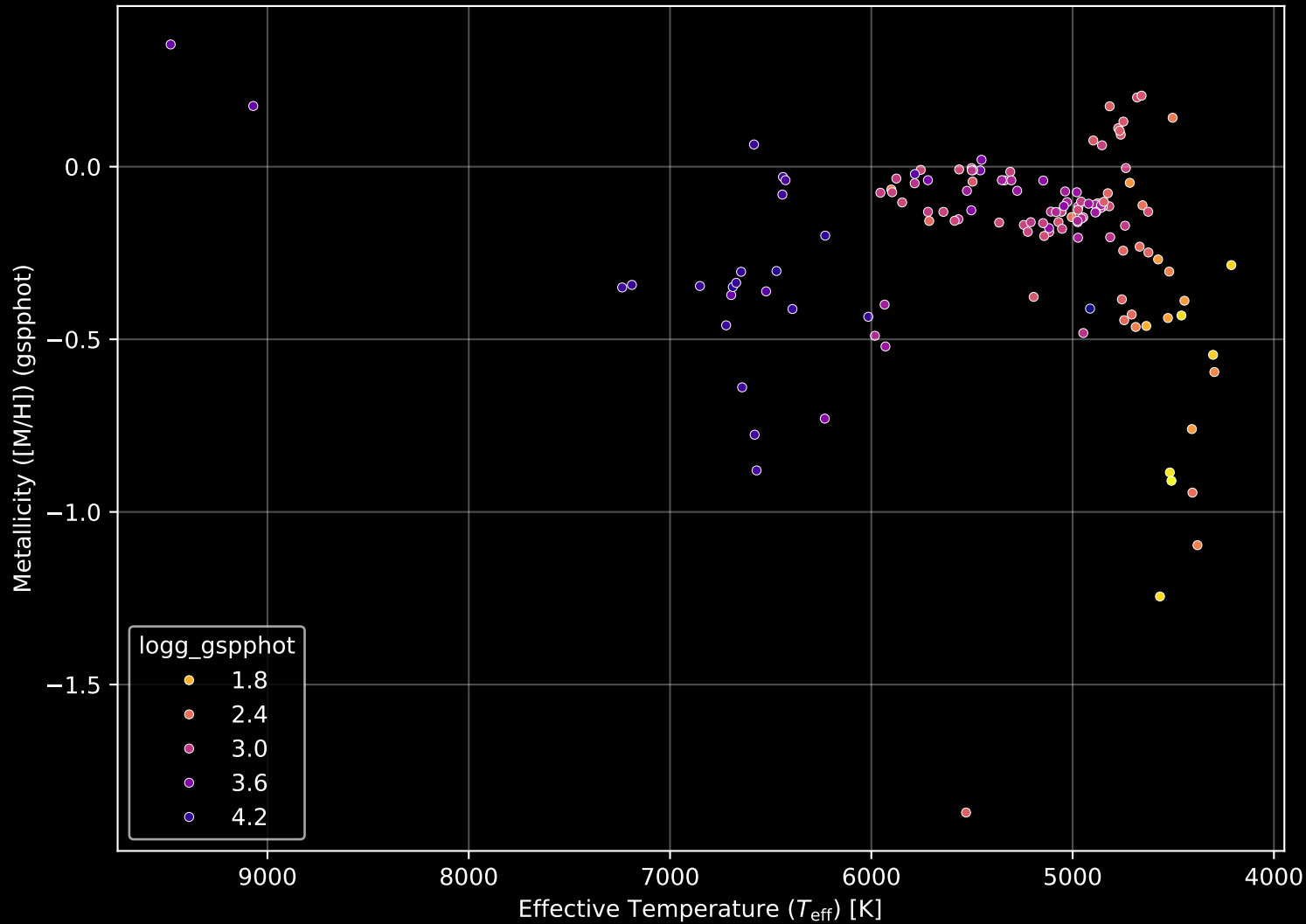
APOGEE DR17 Field: [015+30] Stellar Population Parameters (n= 135)
